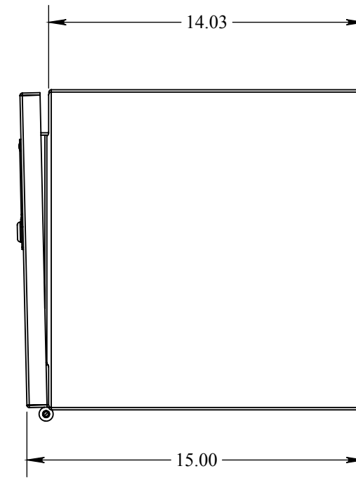
End View
